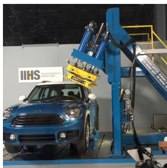
Figure 2. IIHS Roof Strength Test
